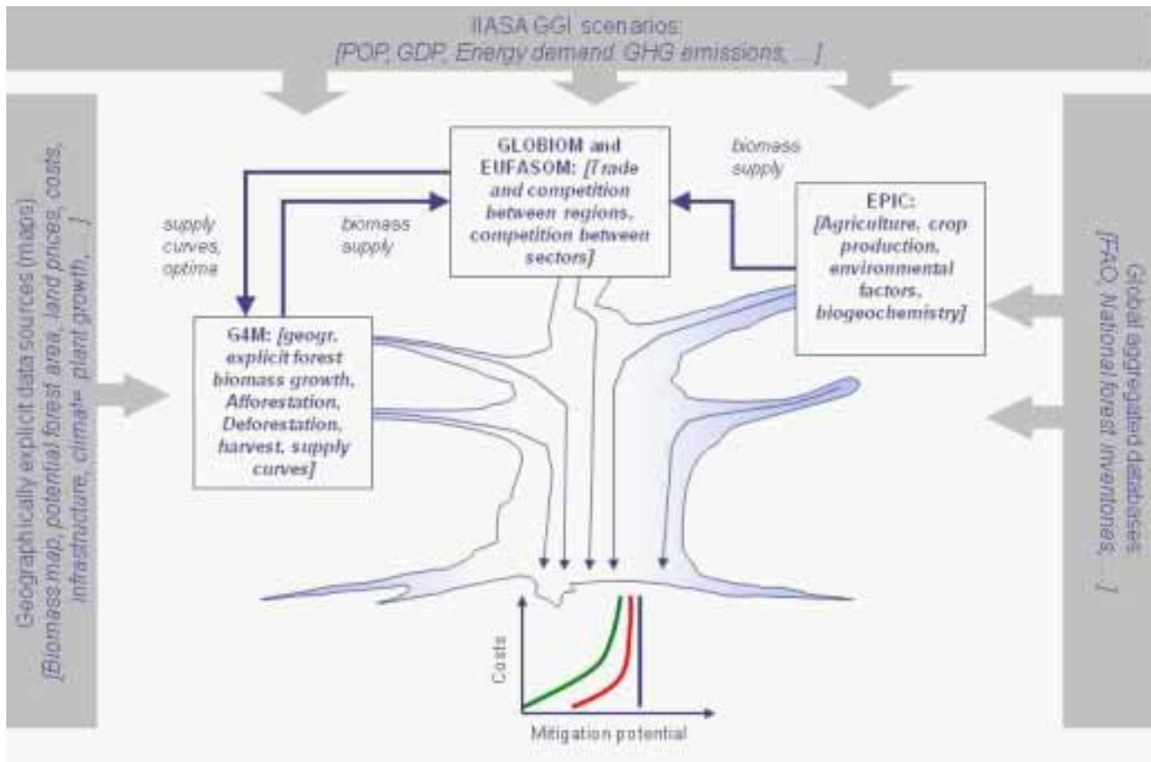
Figure 12: Biophysical/economic model cluster (source: EuroGEOSS)
