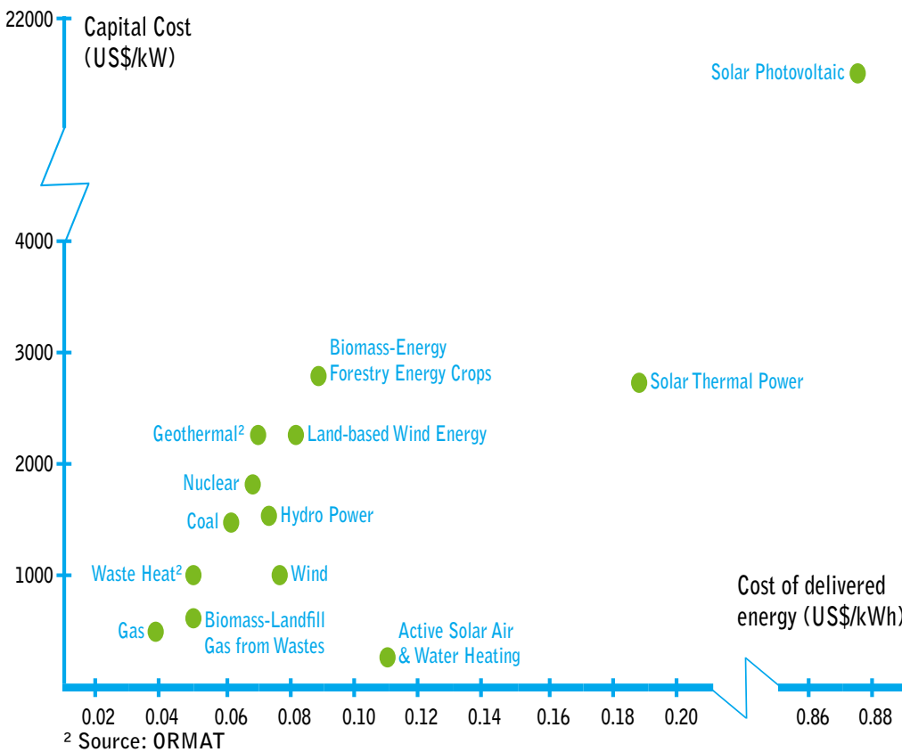
Figure 18: Cost of renewable energy (from: renewable energy projects handbook (WEC), source: the case for renewable energy in emerging markets, W-J van Wijk, CDC, ORMAT)
