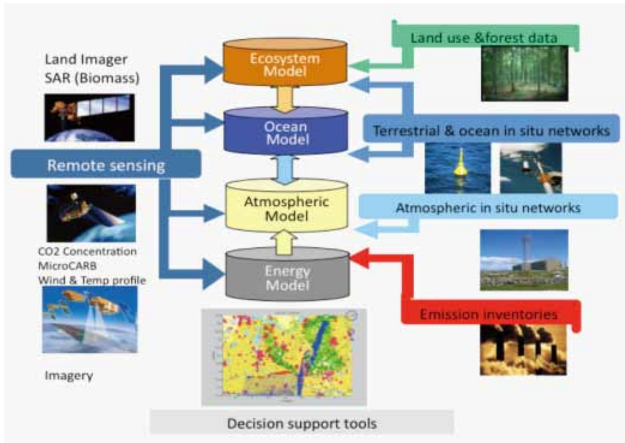
Figure 14: modelling framework (GEO carbon strategy)
