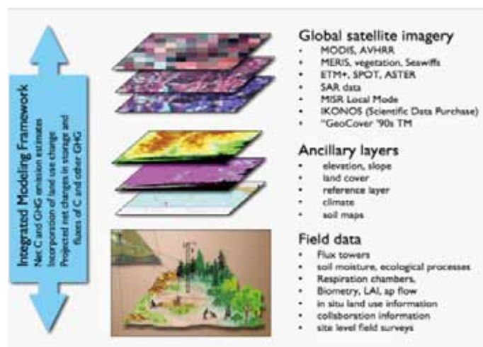
Figure 13: decision support tools (GEO carbon strategy)
